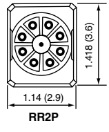
RR Series Relays (pin)
