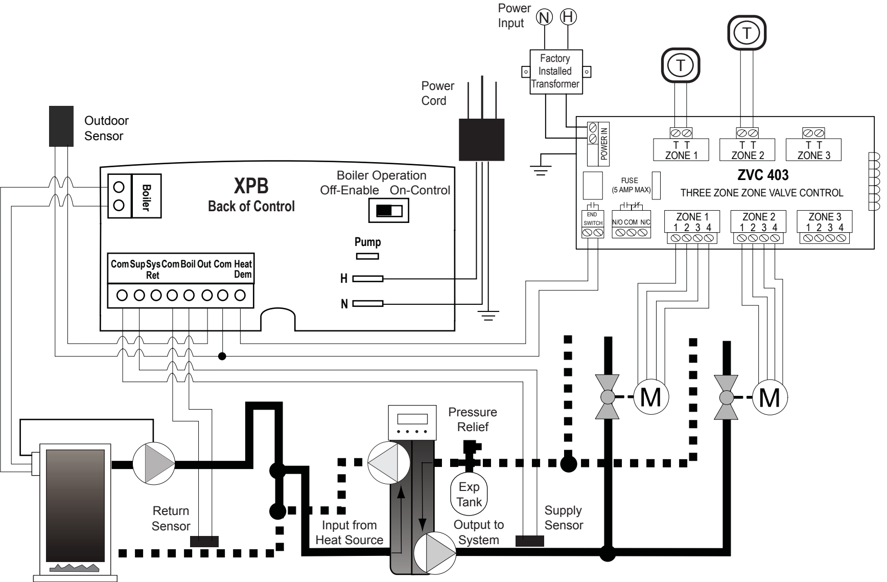
X - Pump Block (XPB), Multiple Zones - Zone Valves
