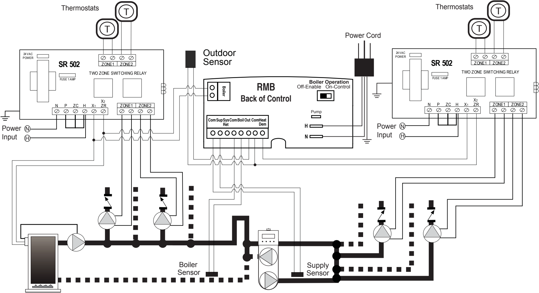
RMB - Radiant Mixing Block, Multiple Temperature System
