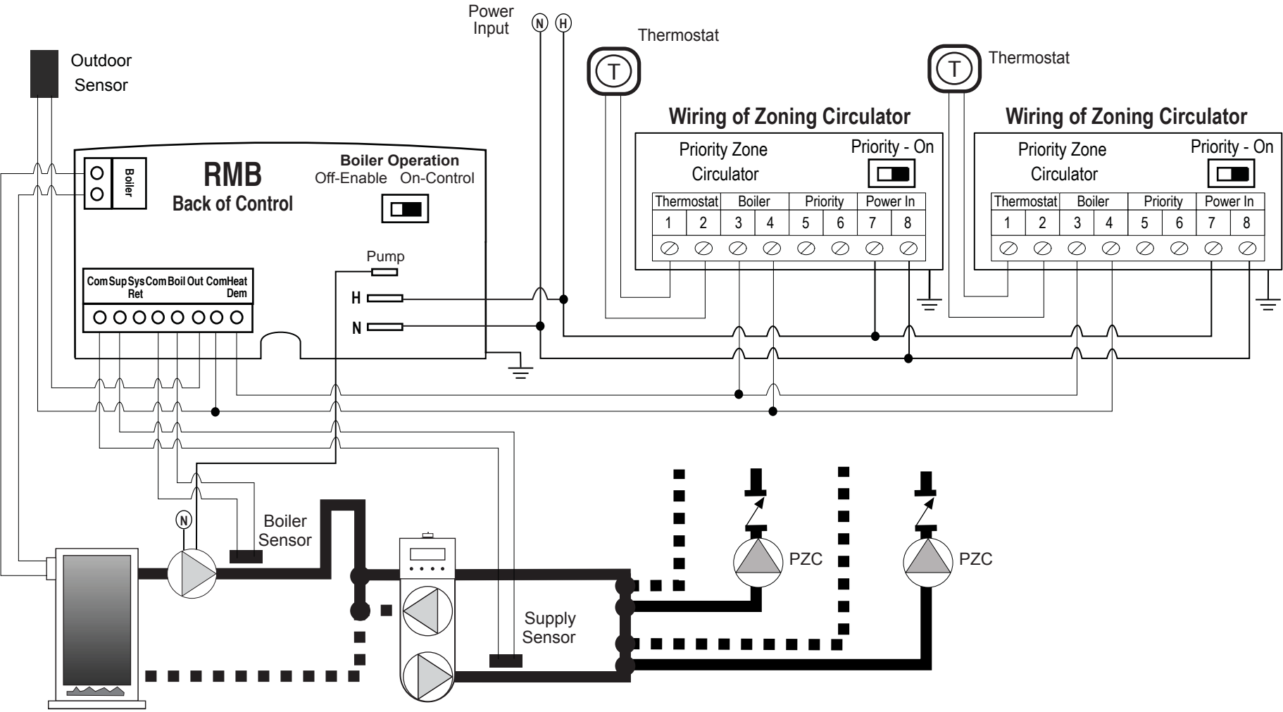
RMB - Radiant Mixing Block, Multiple Priority Zoning Circulators (PZC)
